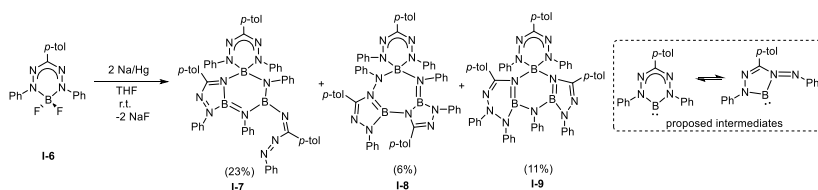
Scheme 1.1.4. Treatment of formazanate \text{BF}_2 with Na/Hg amalgam. 21
