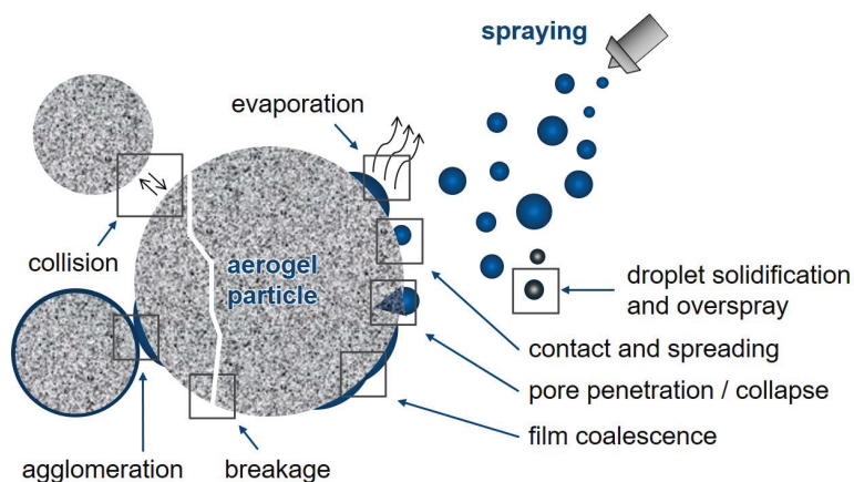
Fig. 1.4: Subprocesses occurring during coating of an aerogel particle.
