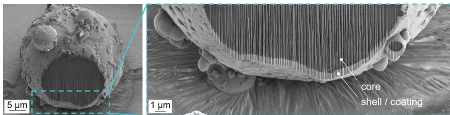
Fig. 1.1: Cross-sectioned aerogel particle with visible core and coating layer.
