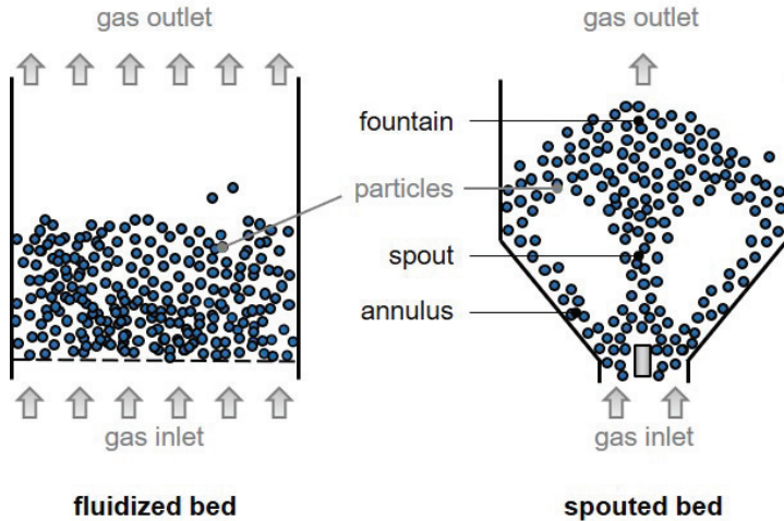
Fig. 2.1: Comparison of the setup of a fluidized (left) and a spouted bed (right).
