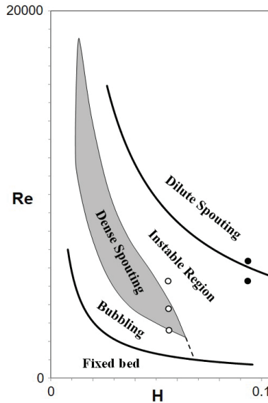
Fig. 2.2: Regime map for of a spouted bed for \gamma\text{-Al}_2\text{O}_3 particles fluidized by air after Salikov et al. [2015].
