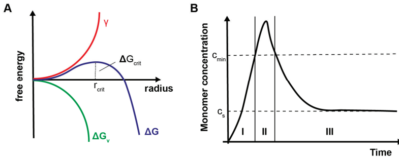
Figure 2.1: Nanoparticle nucleation and growth. (A) Free energy diagram for nucleation. (B) Classic LaMer mechanism for nanoparticle growth. [66]
